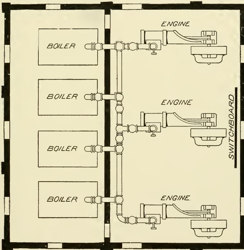
Fig. 144. Diagram of the Principal Elements in a Small Power Station
